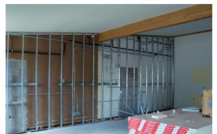
Gypsum Partitions
